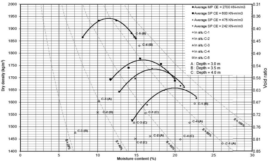
Figure 3. Compaction lab tests and in situ compaction measurements in trial pits C-1 to C-5.
