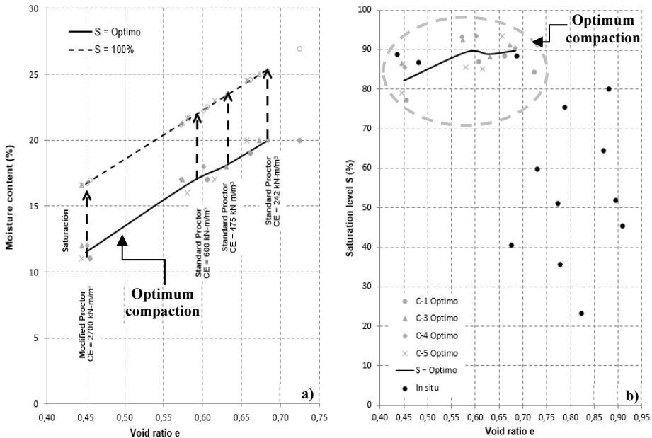
Figure 4. Moisture content vs. void ratio for different compaction energy levels (CE) and saturation ( S ), and in situ conditions according to measurements in trial pits C-1 to C-5.
