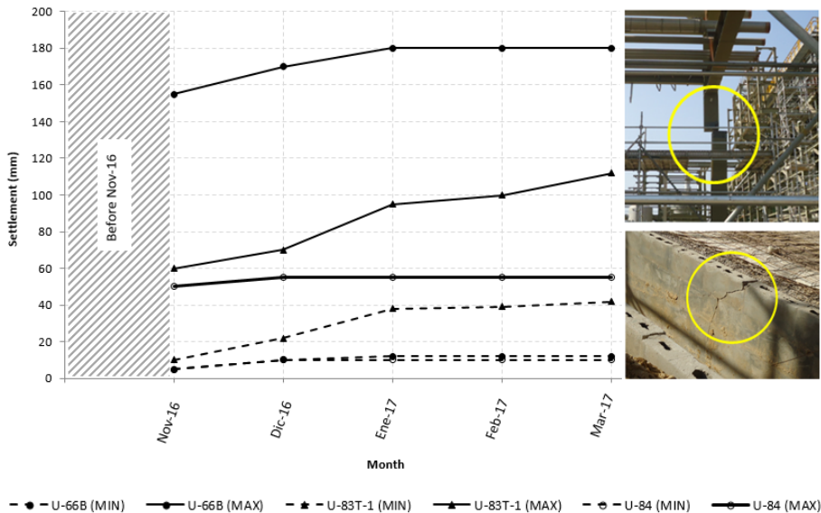
Figure 1. Settlement measurements and field deformations evidences.
