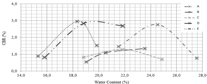
Figure 5. CBR curves.
