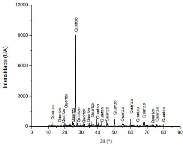
Figure 4. XRD results.
