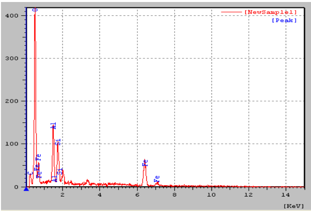
Figure 3. SEM-EDS of sample 2.
