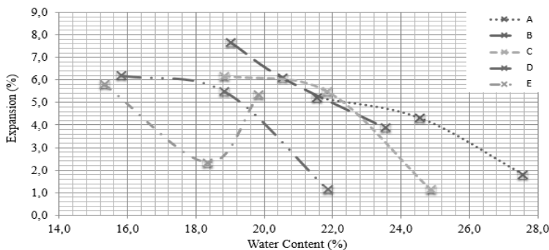
Figure 6. Expansion curves.
