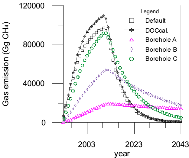
Figure 1. IPCC model using DOC_{\text{default}} and DOC_{\text{calculated}} values.
