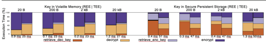
Figure 2. Re-encryption TA microbenchmark
