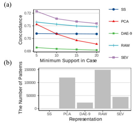
Figure 3: (a) Comparison of the predictive performance of the association patterns discovered using the various data representations as a function of the minimum support in cases (minsupC) (b) The number of association patterns discovered using the various data representations. (minsupC=5)
