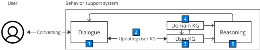
Figure 1. System Architecture.
