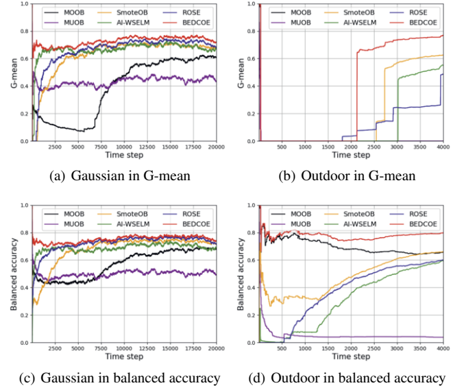
Figure 2. Continuous performance comparison throughout time on representative data sets in terms of G-mean and balanced accuracy.
