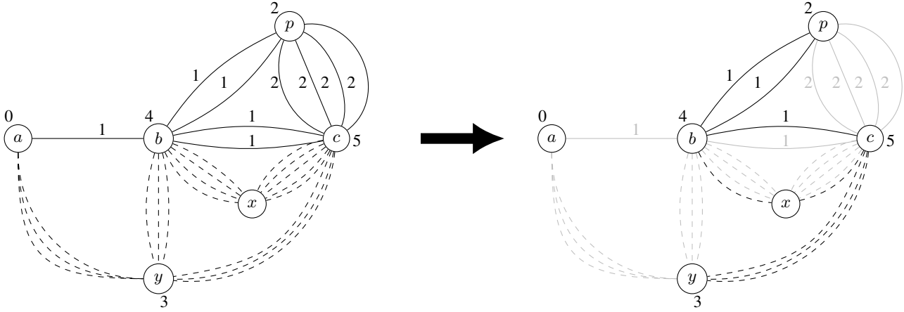
Figure 2. Example of the construction from the proof of Theorem 4 applied to the instance of 2-Veto-Bribery from Example 2 (left) and the perfect b -matching of weight k = 3 corresponding to \widehat{V} (right). In the graph solid edges are labeled with their corresponding weight, dashed edges have weight 0, and each vertex is labeled with its b -value. Recall that a perfect matching corresponds to the complement of the final bribed election. The “grayed out” edges on the right show the final bribed election, which has four voters vetoing p and c , one voter vetoing a and b , one voter vetoing b and c , and three bribe vetoes for a and three bribes vetoes for b (corresponding to the three (a, y) edges and the three (b, y) edges).
