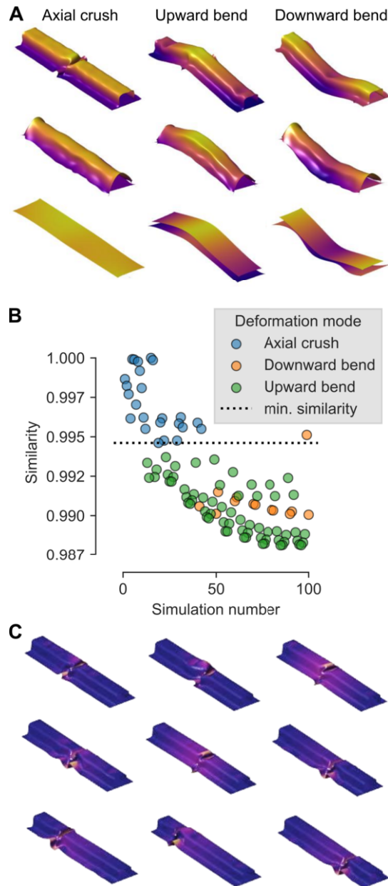
Figure 5. (A) Mesh reconstruction for three deformation modes (color scale indicates displacement in z -direction): top row shows mesh reconstructions from the first 500 eigenvectors ordered by magnitude of eigenvalues; middle row shows reconstruction from the proposed descriptor with sizes M = 14 for axial crush, M = 17 for upward bend, M = 16 for downward bend, bottom row shows reconstruction from the first M = 14 , M = 17 , and M = 16 eigenvectors ordered by magnitude of their eigenvalues. (B) Cosine similarity between axial crush descriptor and all simulation runs. (C) First nine most similar simulation results for axial crush spectral descriptor (color scale indicates displacement in z -direction).
