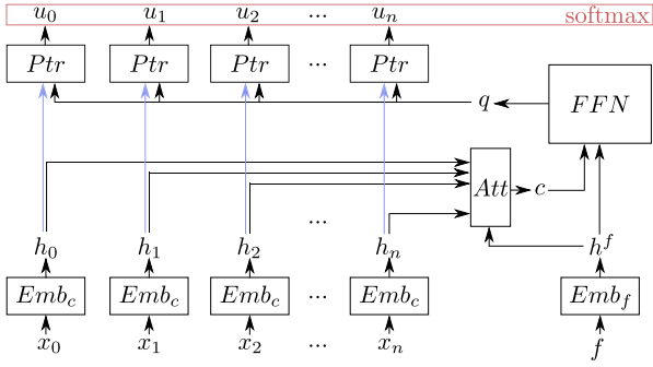
Figure 2. Network architecture
