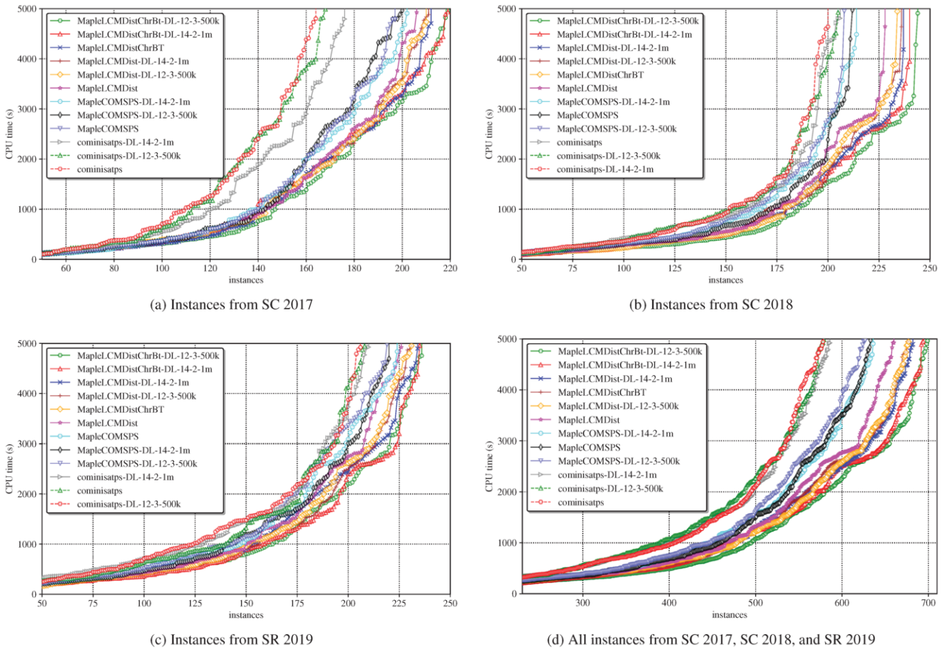
Figure 2. Comparison of the considered solvers on instances from SC 2017, SC 2018, and SR 2019
