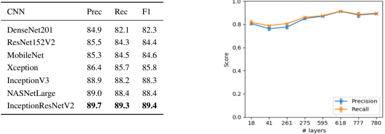
Figure 1. Left: Comparison of models trained using different CNNs as feature extractors. Right: Classifier performance for models trained using features extracted from various points of the InceptionResNetV2 network. All metrics were macro-averaged across classes.
