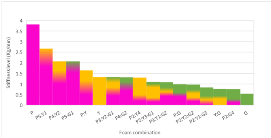
Figure 8. Stiffness as calculated from creep test measurements with a human form indenter probe at 60 kg load. 150 mm total height of cushion layered with different hardness, indicated by P (pink), Y (yellow) and G (green). Numbers represent the thickness ratio of each foam used.
