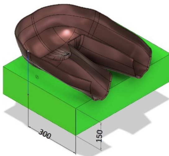
Figure 6. Indenter placement.
