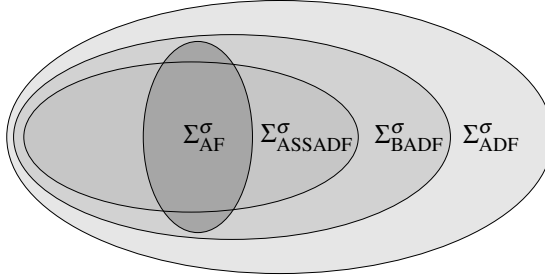
Figure 3. Expressiveness of subclasses of ADFs for \sigma \in \{adm, prf, com\}
