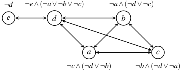
Figure 2. ASSADF without supporting links being not semi-coherent.
