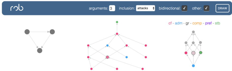
Figure 1. The web interface of Rob. From left to right: the detail of a selected AF, the lattice of all non-isomorphic AFs with three arguments, and the lattice of the extensions for the selected AF.
