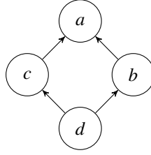
Figure 2. The argumentation framework from Example 3
