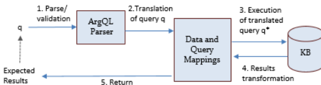
Figure 1. Process of query execution
