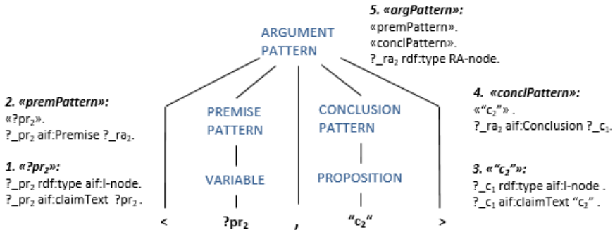
Figure 2. Part of the translation process of q
