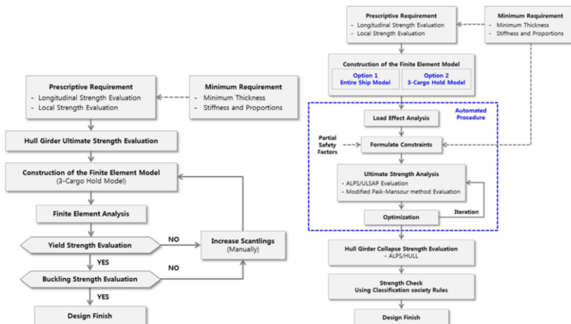
Figure 2: Approaches for the design of preliminary hull structural scantlings; a) Industry standard (IACS 2012) b) Optimization approach proposed by Kim & Paik (2017)
