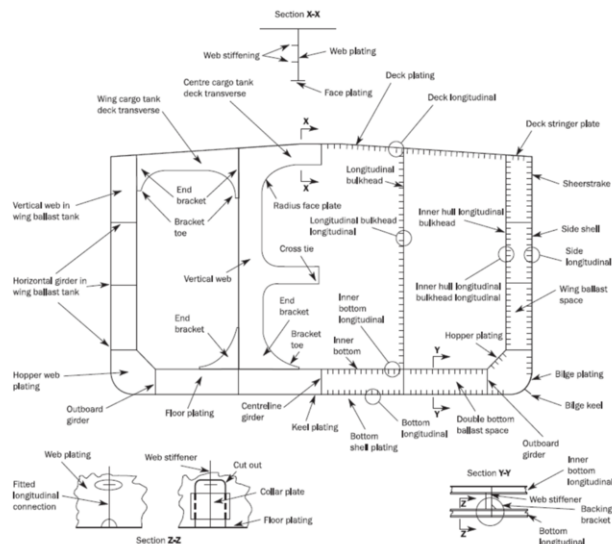
Figure 23: Mid cargo hold transverse section of double hull tanker (CSR BC & OT, IACS(2017))
