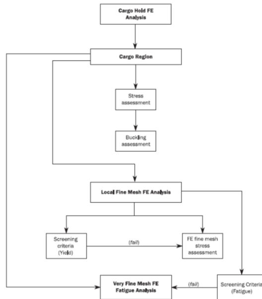
Figure 24: Flow diagram of finite element analysis (CSR BC & OT, IACS (2017))
