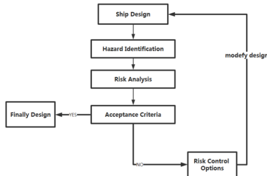
Figure 3: Risk - based ship design flow chart
