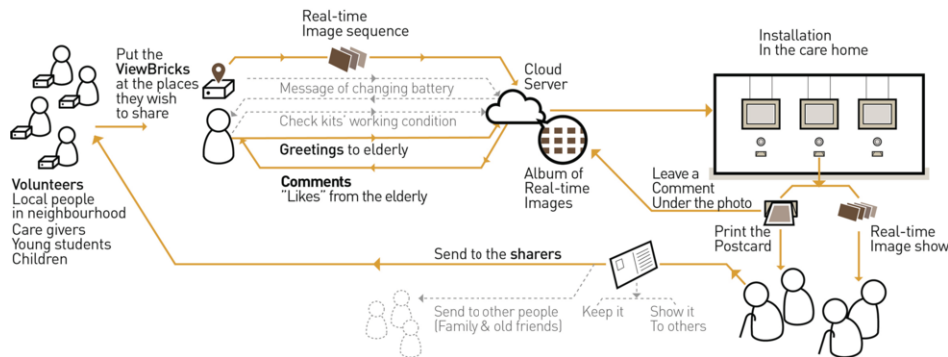
Figure 1. Structure of ViewBricks System.
