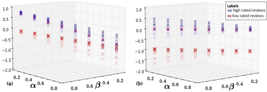
Figure 1. Scores of each review for a single hotel. A red cross denotes a review that belongs to Low and a blue circle denotes a review that belongs to High. (a) Scores vs \alpha and \beta aggregating using ArgAll (b) Scores vs \alpha and \beta aggregating using AttSupBoth . Both use f_{max} .
