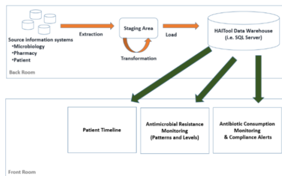
Figure 1. HAITool's architecture.
