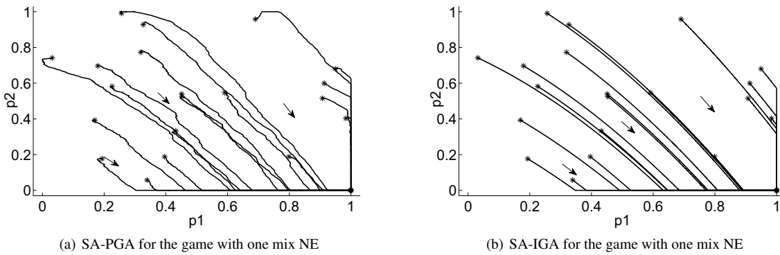
Figure 3: The Learning Dynamics of SA-IGA and SA-PGA in game with one mix NE (parameter w_r(0) = w_c(0) = 0.85 , \delta_p = 0.001 , \alpha = 0.8 and \varepsilon = 0.02 )
