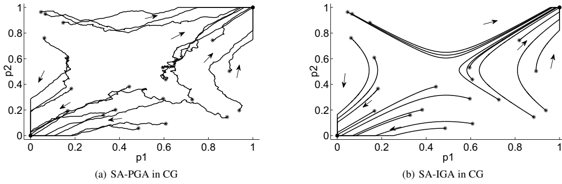
Figure 2: The Learning Dynamics of SA-IGA and SA-PGA in coordination game (parameter w_r(0) = w_c(0) = 0.85 , \delta_p = 0.001 , \alpha = 0.8 and \varepsilon = 0.02 )
