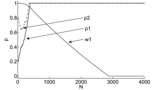
Figure 5: SA-PGA against a selfish agent for in coordination game( w_r(0) = 1 , p_r(0) = 0.2 and p_c(0) = 0.8 )
