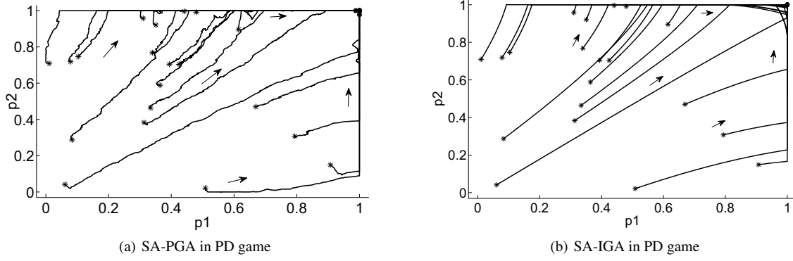
Figure 1: The Learning Dynamics of SA-IGA and SA-PGA in PD game (parameter w_r(0) = w_c(0) = 0.85 , \delta_p = 0.001 , \alpha = 0.8 and \varepsilon = 0.02 )
