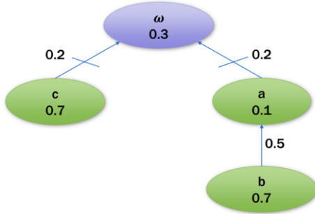
Figure 1. An example of a WBAF, as specified in Example 1. Nodes represent the arguments, arrows indicate attacks and arrows with diagonal lines indicate support. The numbers within the nodes represent the belief function and the numbers next to the edges represent the weighing function.
