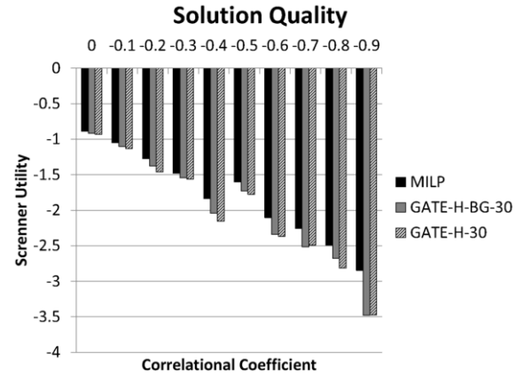
Figure 7. Solution Quality - Moving to Zero Sum
