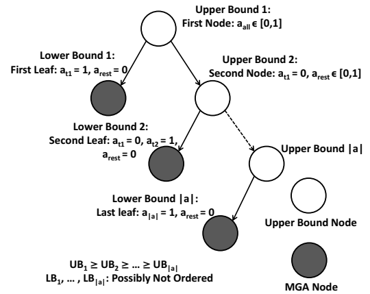
Figure 3. Branch-and-Guide Tree
