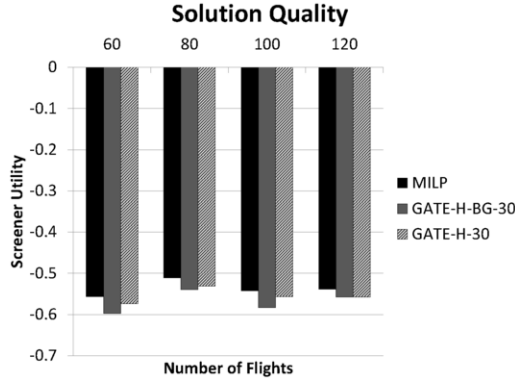
Figure 5. Solution Quality - MILP and GATE
