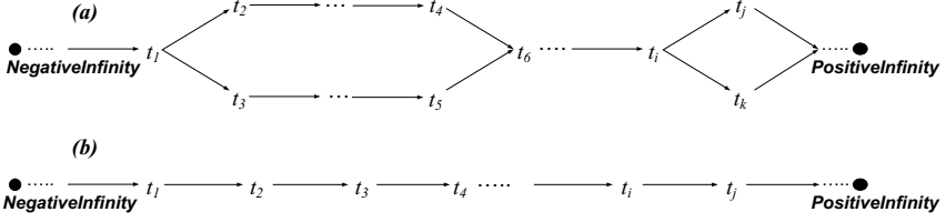
Figure 1. Time models of SUMO with instants connected by relation before .
