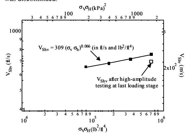
Figure 5. Effect of increasing total static vertical and horizontal stresses on S_{hv} -wave velocities at a depth of 18 cm beneath the footing
