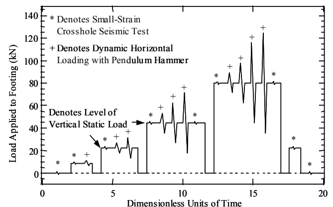
Figure 4. Schematic illustration of the testing sequence used in the small-strain (linear) and large-strain (nonlinear) shear wave measurements
