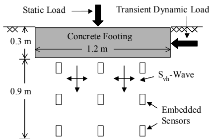
Figure 1. Basic approach for performing nonlinear shear modulus measurements
