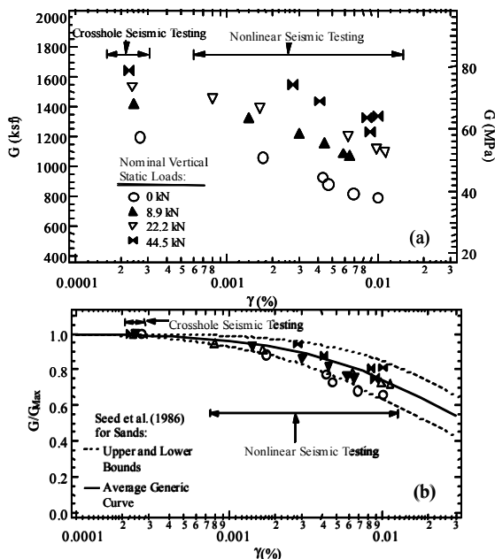
Figure 6. In-situ measurements of the : (a) G - \log \gamma and (b) G/G_{max} - \log \gamma relationships at an average depth of 11 cm beneath the footing
