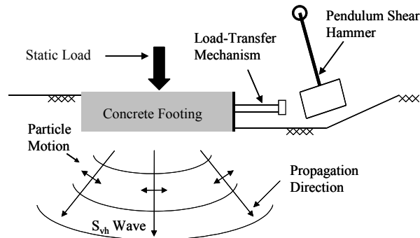
Figure 3. Generation of linear and nonlinear S_{vh} waves using a pendulum hammer
