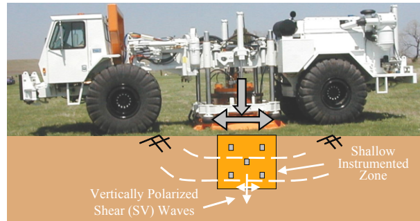
Figure 7. Illustration of new dynamic source (T-Rex) loading an instrumented site
