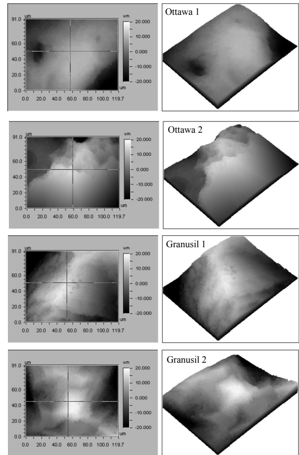
Figure 2. Graphical representation of data obtained for Ottawa and Granusil® sands
