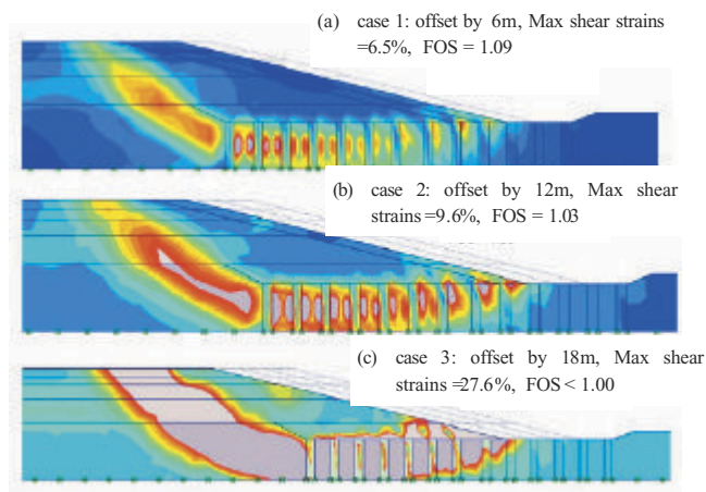
Figure 3 Shear strains for 7.5m bund with bund alignment offsets by (a) 6m (b) 12m and (c) 18m
