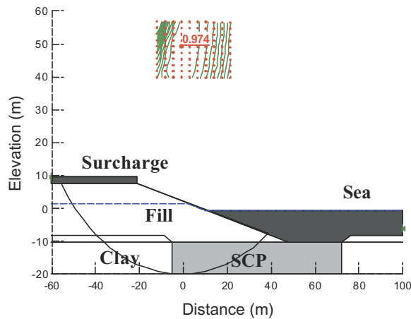
Figure 2 Failure of bund slope under a combination of adverse conditions
