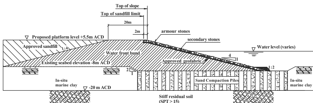
Figure 1 Typical water front bund design scheme
