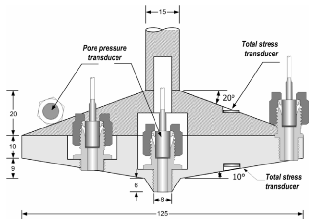
Figure 14. Model spudcan
