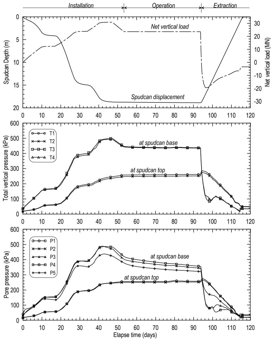
Figure 17. Time records of a typical spudcan extraction test
