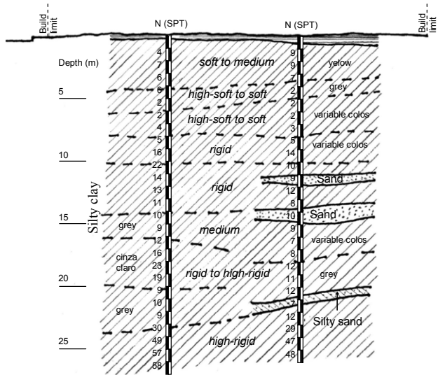
Figure 2 – Geologic profile of local subsoil
