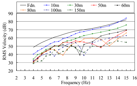
Figure 4. Vibration velocity amplitude in z-dir. in the vertical test.
