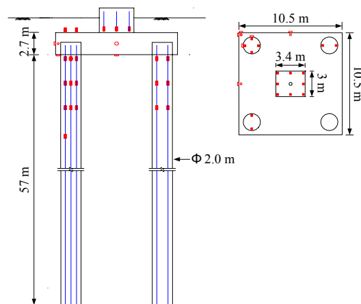
Figure 1. The profile (left) and plan view (right) of the pile foundation(CECI, 2001).
