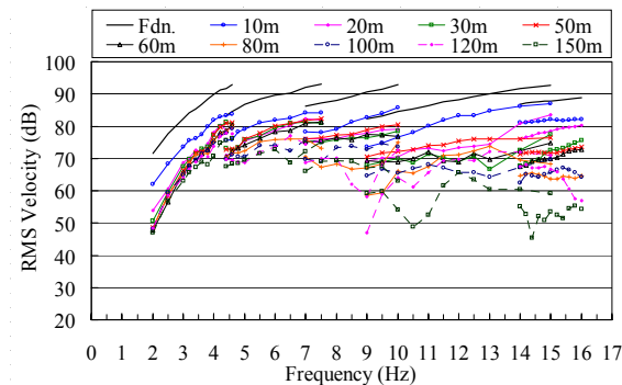
Figure 3. Vibration velocity amplitude in x-dir in the horizontal longitudinal test.
