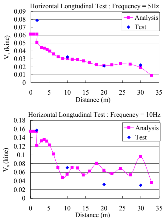
Figure 9. Ground velocity amplitude in x-direction in horizontal longitudinal test (top: 5 Hz; bottom: 10Hz).
