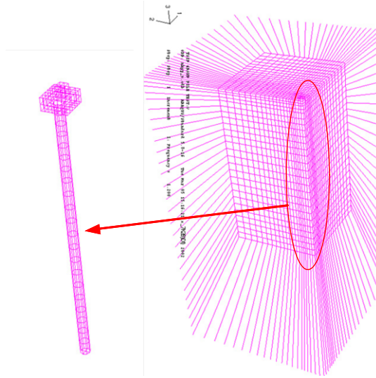
Figure 6. The FEM mesh used in numerical analysis.
