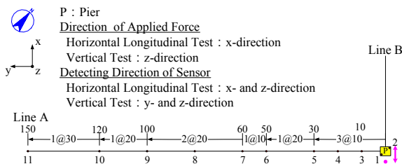
Figure 2. Layout of measuring points during the test.
