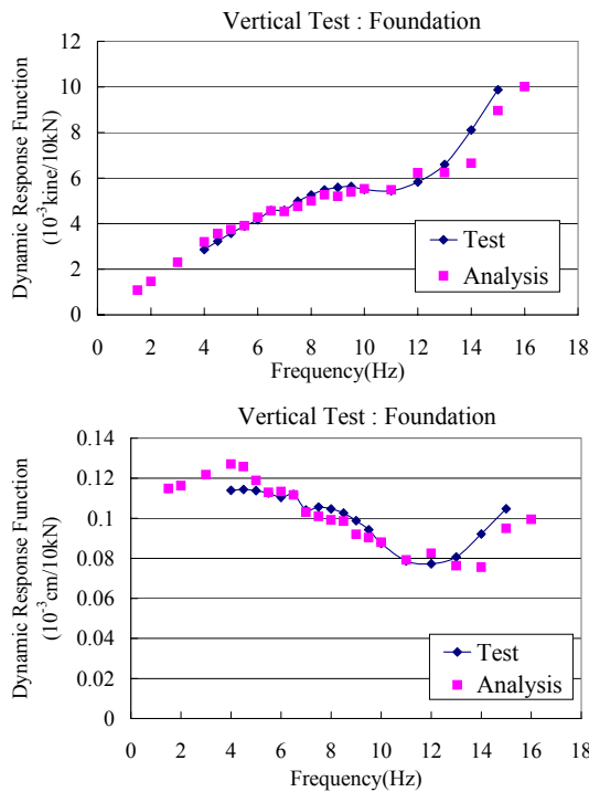
Figure 8. Dynamic response function in z-direction in vertical test (top: velocity; bottom: displacement).
