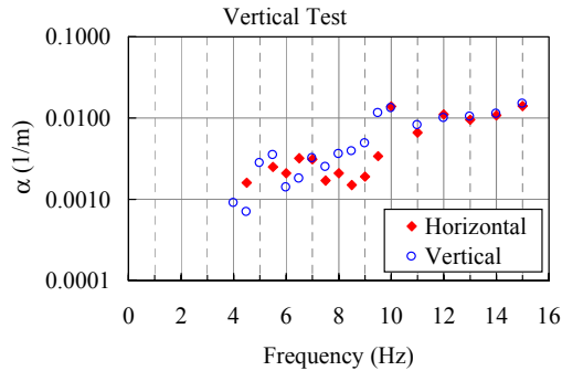
Figure 5. Attenuation coefficient of ground vibration in the vertical test.
