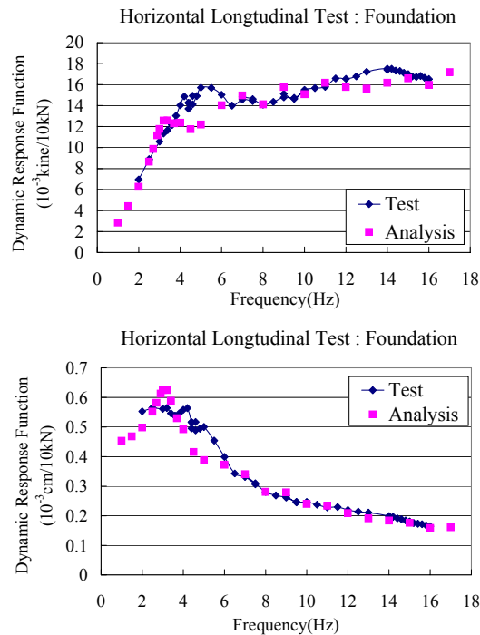
Figure 7. Dynamic response function in x-direction in horizontal longitudinal test (top: velocity; bottom: displacement).
