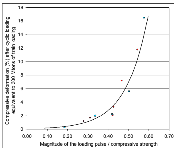
Figure 8. Effect of the magnitude of the loading pulse compared to the compressive strength of board on the compressive deformation of XPS frost insulation boards in a cyclic loading test corresponding to a train loading of 300 million tons.
