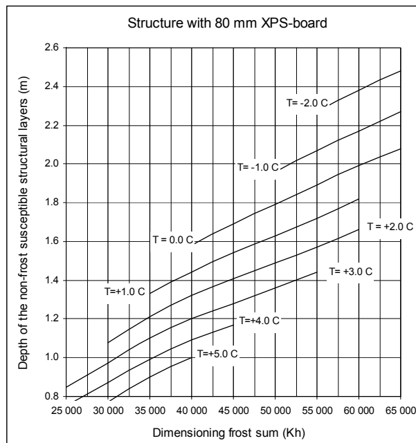
Figure 6. Track frost dimensioning curves based on the 0.050\text{ W/Km} dimensioning value of the XPS insulation board with an insulation thickness of 80 mm. T stands for the annual average temperature of air in the region. (Nurmikolu & Kolisoja, 2002)
