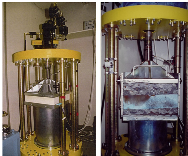
Figure 7. A regular cyclic loading test setting (left) and a setting where the loading is applied to the insulation board through a ballast layer (right).
