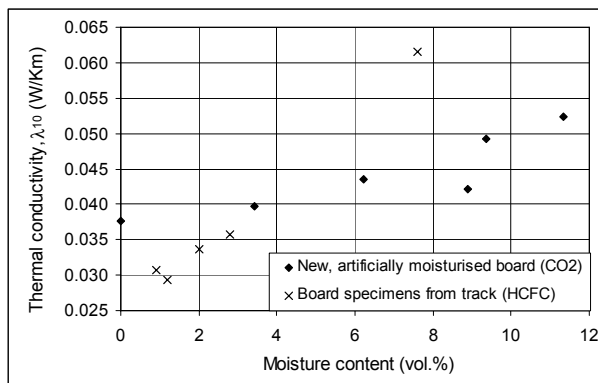
Figure 5. Results of thermal conductivity measurements ( \lambda_{10} ) on XPS boards removed from a track structure representing the earlier technology where HCFC was used as a blowing agent and boards made using \text{CO}_2 as a blowing agent (Styrodur C-RHS) and moisturised artificially.
