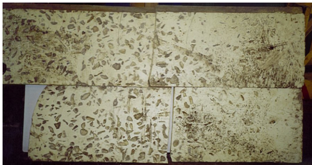
Figure 4. A typical example of indentations caused by ballast grains on the bottom surface of an XPS board.
