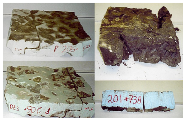
Figure 3. Mechanical damage in XPS frost insulation boards, generally (left), and in the problematic production lot (top right). An example of cracks in the bottom surface of a board, bottom right.
