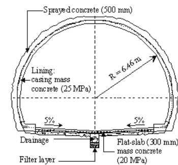
Figure 1. Original cross-section of the tunnel
