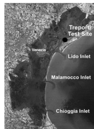
Figure 1. Satellite view of the Venetian Lagoon, with location of the Treporti test site.
