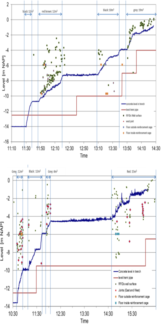
Figure 2. Relation between scanned level RFIDs and concrete level at time of insertion for panels 1 and 2.
