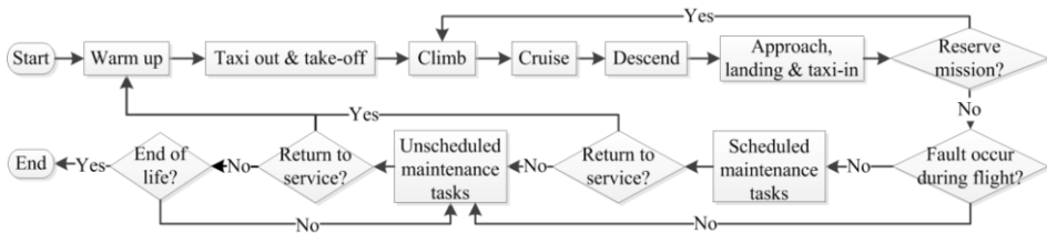
Figure 2 Operation & maintenance process model
