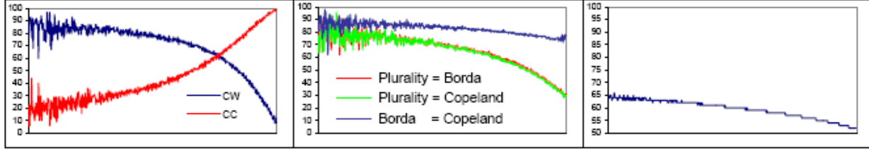
Figure 2. Diversity for \Delta^{\Sigma,K}_{dist} / IC data ( x -axis). Condorcet winners/cycles; agreement between voting rules; voter satisfaction ( y -axis). [ n = 50, m = 5 ]
