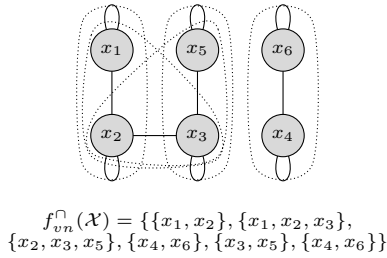
Figure 3: f_{vn}^\cap illustration.
