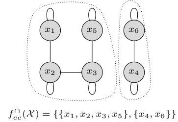
Figure 2: f_{cc}^{\cap} illustration.
