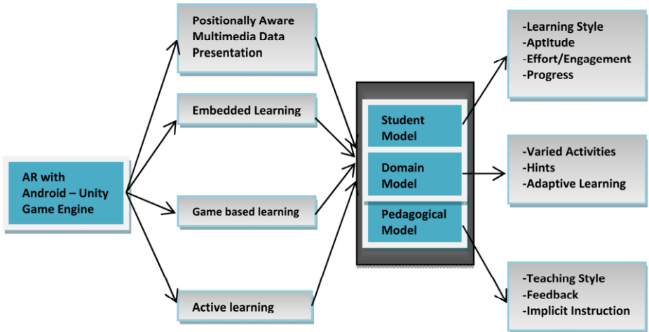
Figure 1. The architecture of AmonPlanet Game
