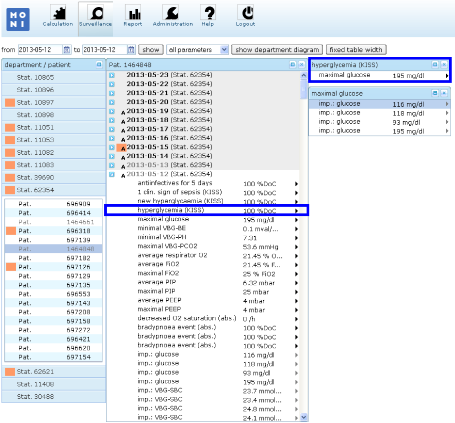
Figure 1. MONI-NICU cockpit view with NEO-KISS criteria (wards and patients were anonymized; wards and patients are listed on the left hand side of the screen. In the middle part, the number of days of the patient’s NICU stay are shown with one day opened, final as well as intermediate, and some raw data are shown beneath the opened day). An explanation for one derived clinical concept—in this case hyperglycemia—is provided on the right side.
