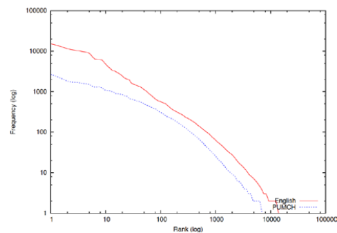
Figure 1- Zipf's distribution of vocabularies
