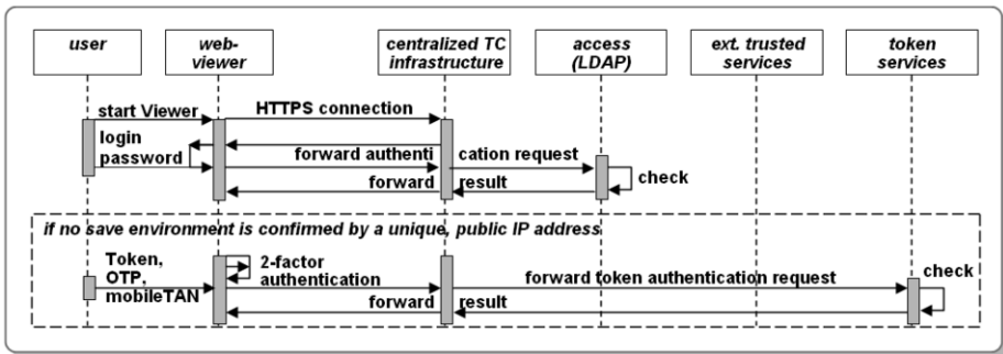
Figure 2. Two-factor authentication.
