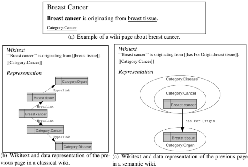
Figure 1. Representation of wiki page about breast cancer (a) in a classical (b) and in a semantic wiki (c).
