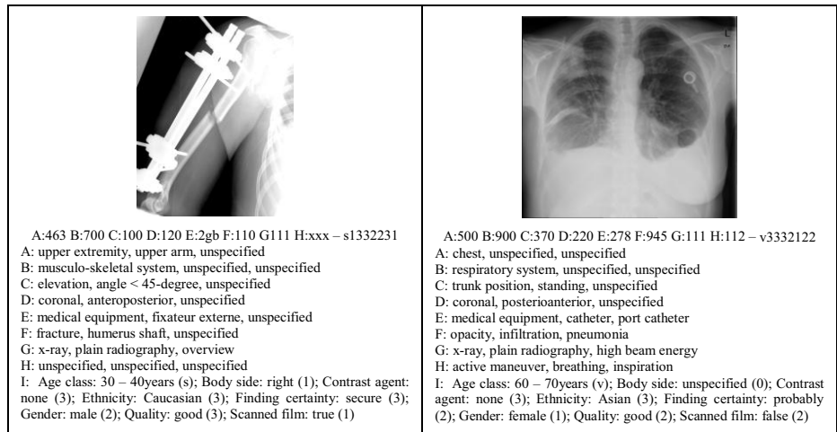
Figure 1: Example images labeled with IRMA Code II
