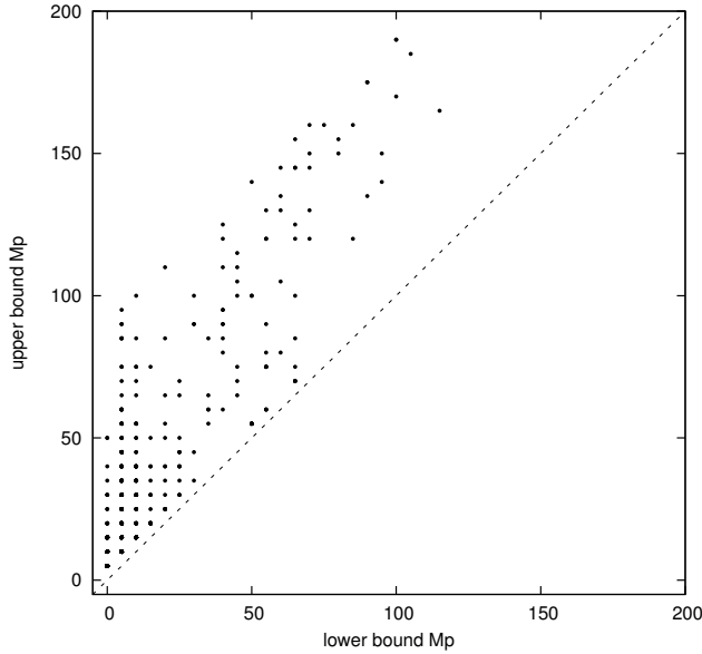
Figure 2. Lower and upper bounds of plan lengths
