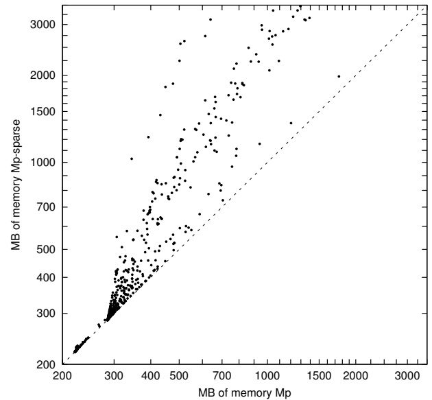
Figure 5. Comparison of memory consumption
