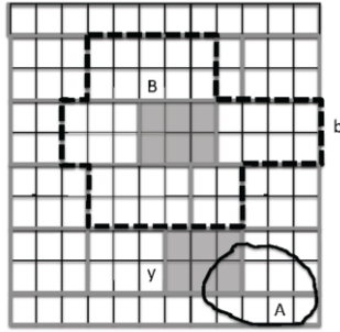
Figure 2. Counterexample for left-to-right direction in prox. cond. (2a)
