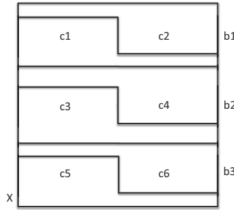
Figure 1. A total order of three partitions: (c_i)_{i \in \{1,2,3,4,5,6\}} \leq (b_i)_{i \in \{1,2,3\}} \leq (X)
