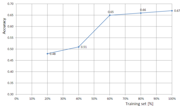
Figure 3. EDITS learning curve on Debatepedia data set
