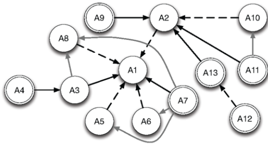
Figure 2. The AF built from the results of the TE module for the debate about “Internet access as a right”. Grey attacks are type 1 attacks introduced to compute the set of accepted arguments. For clarity of the picture, we visualize only a subset of type 1 attacks.
