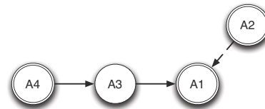
Figure 1. The AF built from the results of the TE module for Example 1, 2 and 3, without introducing entailment attacks. Plain arrows represent attacks, dashed arrows represent entails.
