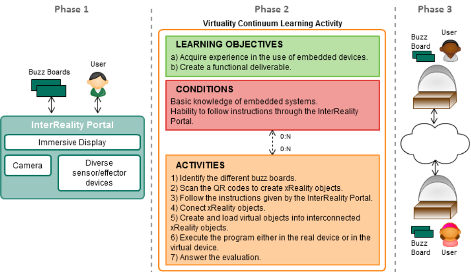
Figure 8. Implementation phases.
