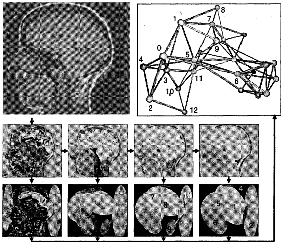
Figure 2 - Image, partitioning, blobs and resulting graphs
