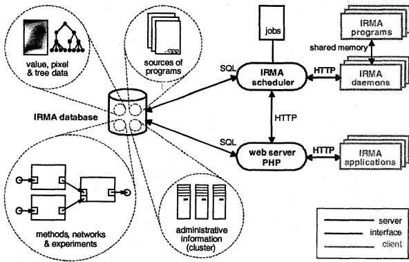
Figure 3 - System architecture
