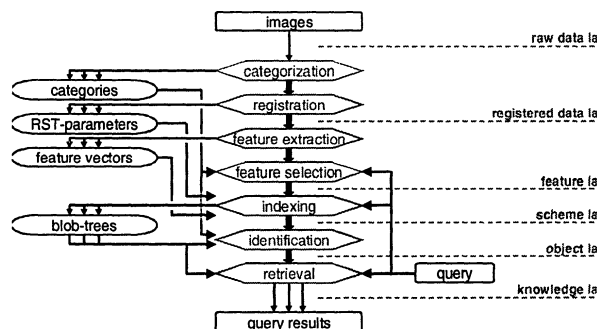
Figure 1 - Processing schemes and semantic layers
