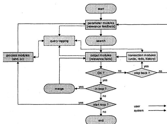
Figure 5 - Extended query refinement
