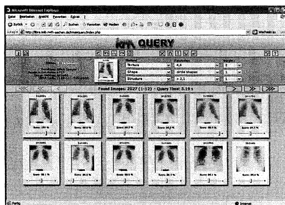
Figure 6 - IRMA query interface
