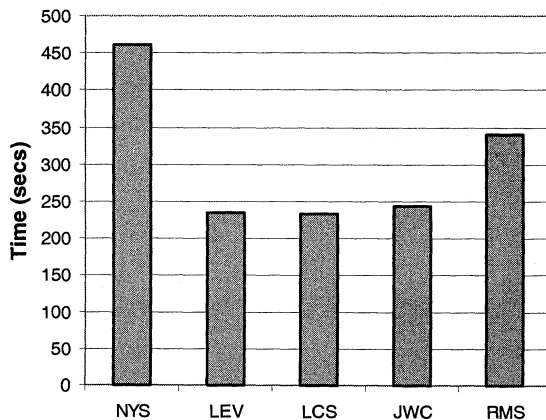
Figure 2 - Total average processing time for 50,000 record pairs
