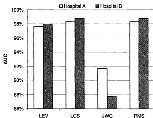
Figure 1 - String comparator accuracy as measured by the area under the ROC curve (AUC) for hospitals A and B
